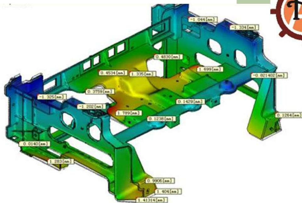
Mold Flow Analysis
