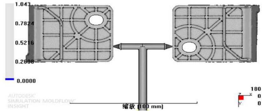
Mold Flow
